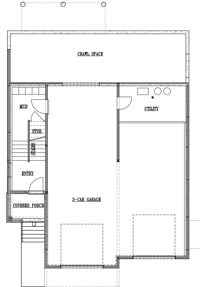
BASEMENT
